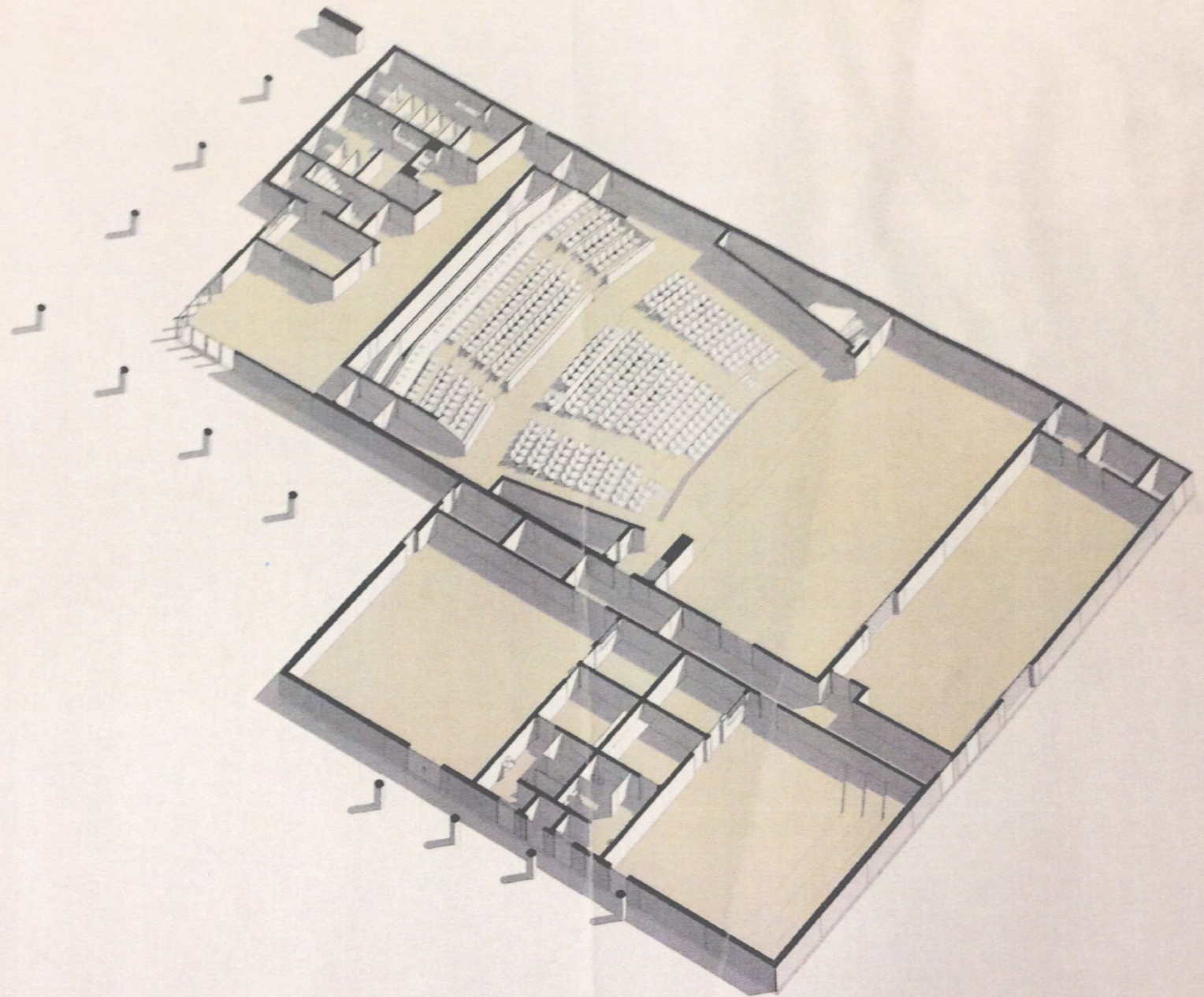
CHRISTIAN BROTHERS HIGH SCHOOL THEATER FIRST FLOOR PLAN
